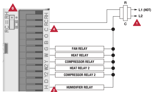
Typical 2H/2C System with Dehumidify Terminal
